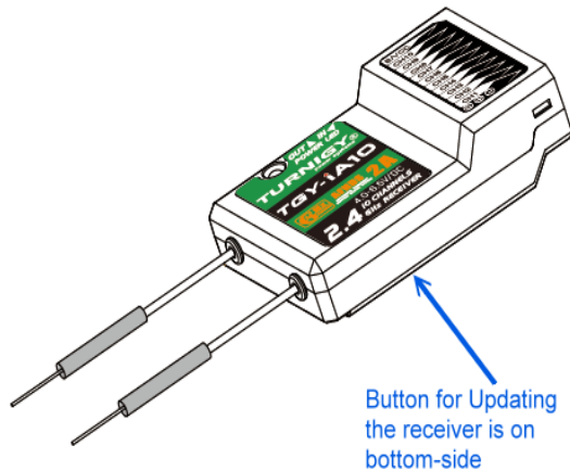
TGY-i10 receiver
