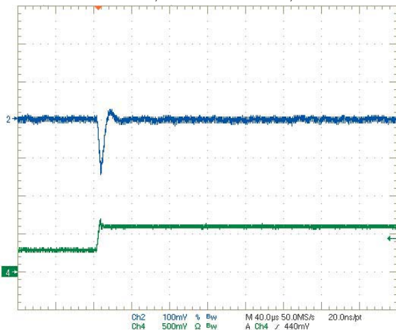
Step Load Transient Response (Vin=12V, Vout=0.591V, Cload=0, Iout=1.5A to 3A) Trace 2=Vout, 50 mV/div. Trace 4=Iout, 1A/div.
