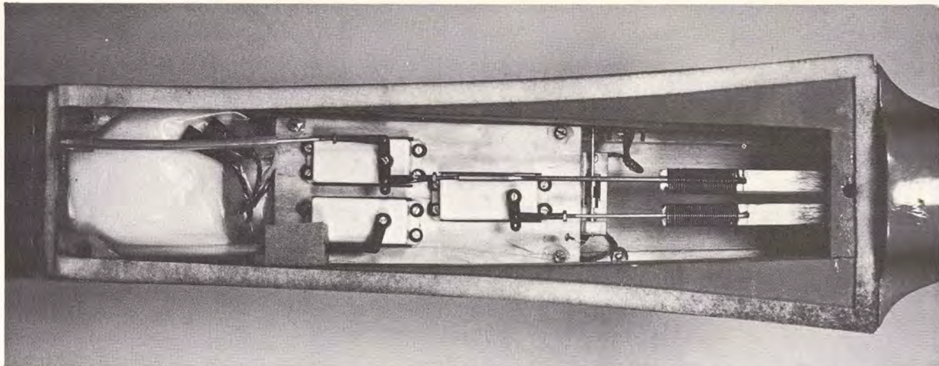
A look inside the fuselage discloses plenty of room to accommodate all the required essentials—note jam nut used to lock Quik-links.
