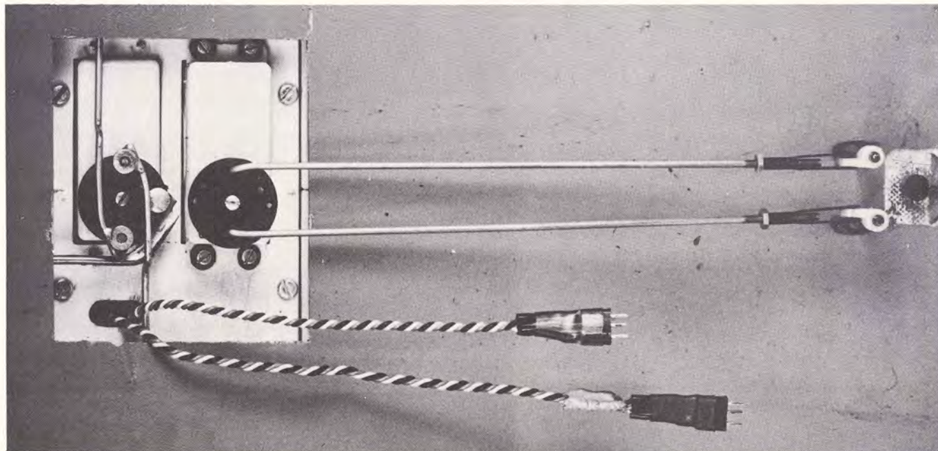
Close-up of aileron and retract servos—Z bend used for aileron pushrods, and over and under method for 180 degree retract linkage.
